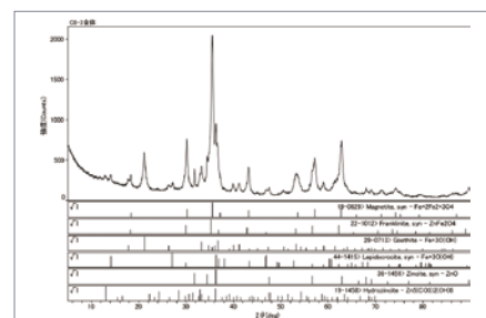
XRD(X線回折)
