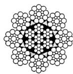
OF IWRC 8 x S (19)
