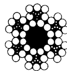
6 x F{(3 x 2 + 3) + 7}
