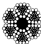
6 x F{(3 x 2 + 3) + 12 + 12}
