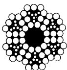
6 x F{(3 x 2 + 3) + 9}
