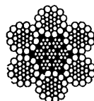
CFRC 6 \times WS(31)
