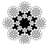
8 x 7 + 8 x WS (31)
